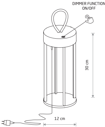
NALA LED painted aluminum, plastic PC
